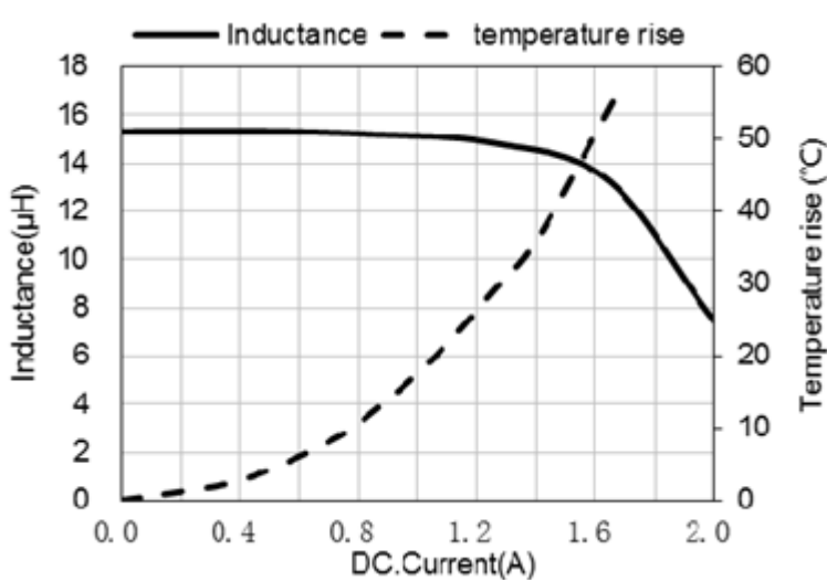
ASPIAIG-S4035-150
