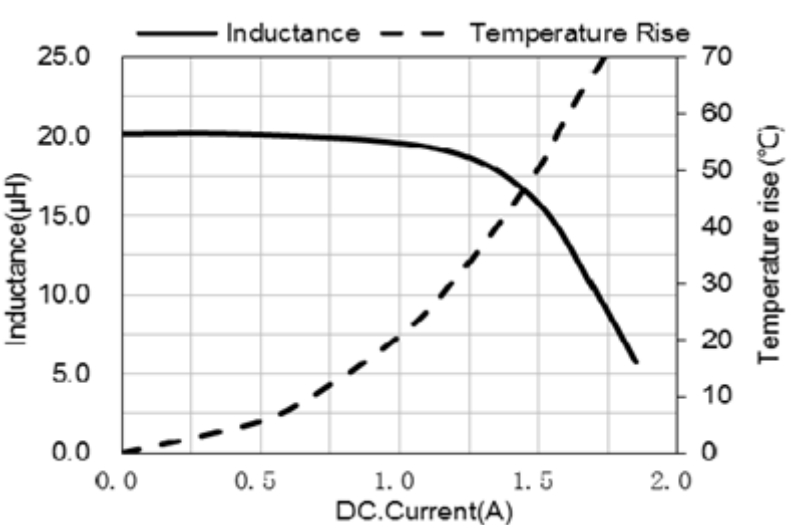
ASPIAIG-S4035-220
