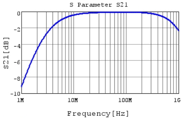
DE1B3RA681KN4AN01F S21 DCOV, 20degC
