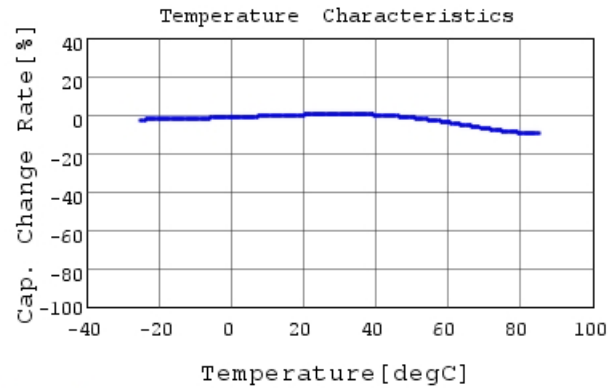
DE1B3RA681KN4AN01F C-Temp. capchange, DCOV,
