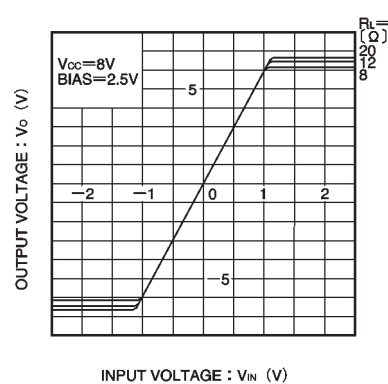
Fig.10 Driver I/O characteristics (channel 3) (during load regulation)
