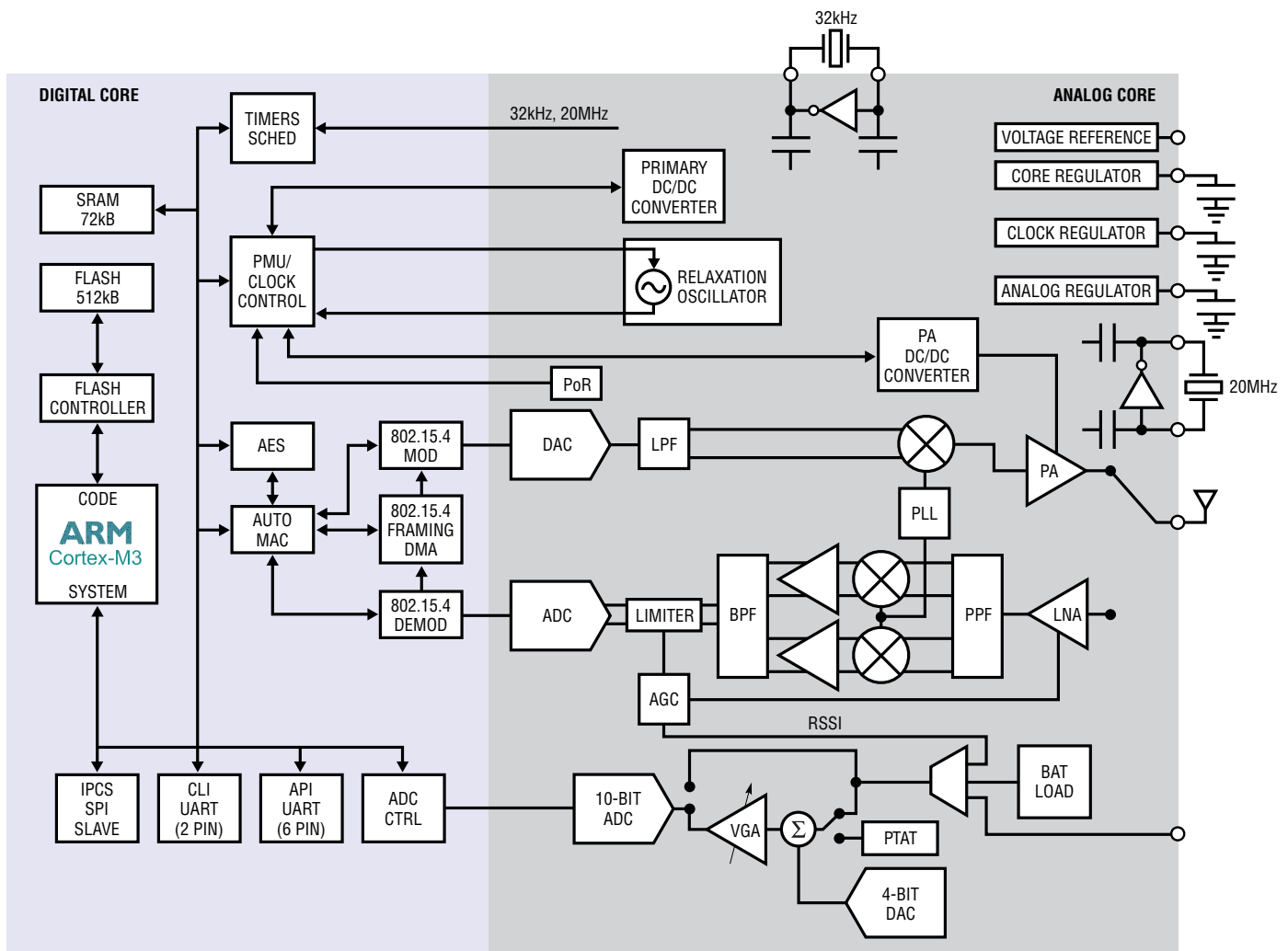
Figure 10. Eterna Block Diagram
