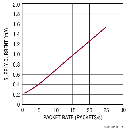
Figure 7a. Supply Current vs Packet Rate
