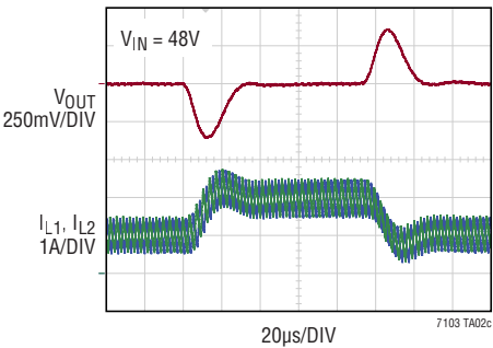
Load Transient
