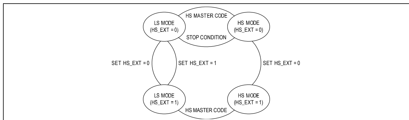
Figure 19. Engaging HS-Mode
