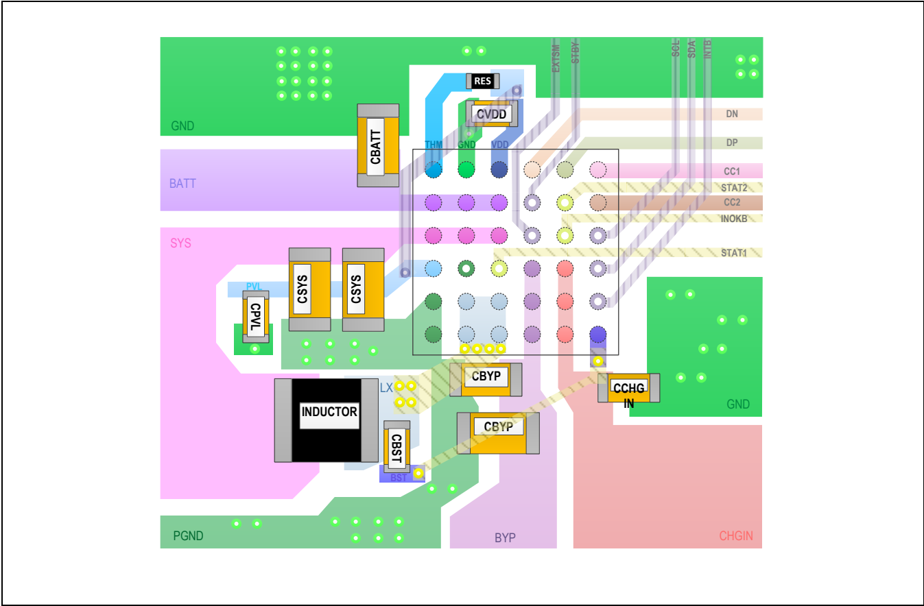
Figure 22. Recommended Placement and Layout
