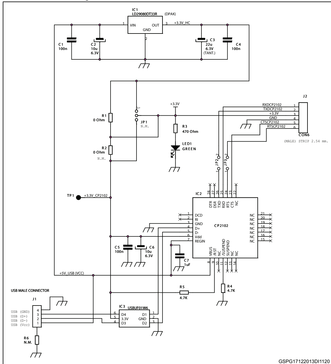
Figure 1. STEVAL-PCC018V1 circuit schematic
