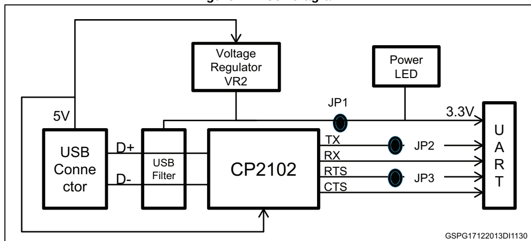
Figure 3. Main components
