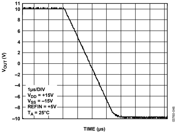
Figure 28. Settling Time
