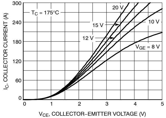
Figure 2. Typical Output Characteristics ( T_C = 175^\circ\text{C} )
