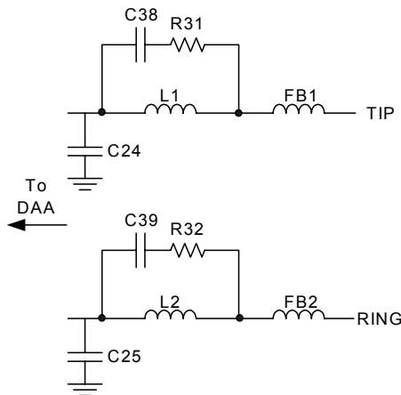
Figure 38. Notch Filter for CISPR22 Compliance
