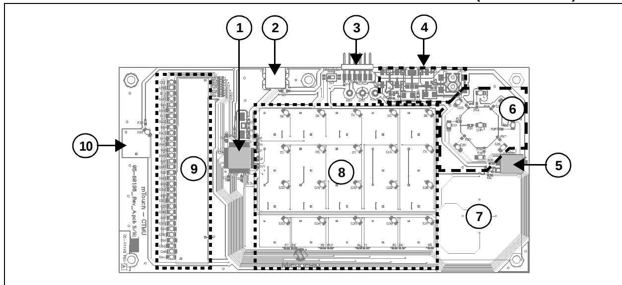
FIGURE 4-3: TOUCH SENSE 2 DEMO BOARD COMPONENT LAYOUT (BOTTOM SIDE)
