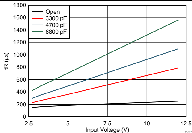
Figure 24. Rise Time vs Input Voltage
