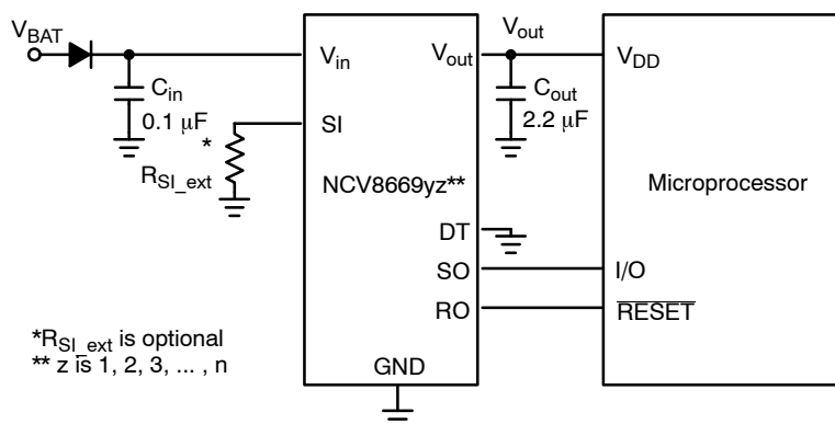
Figure 1. Application Circuit
