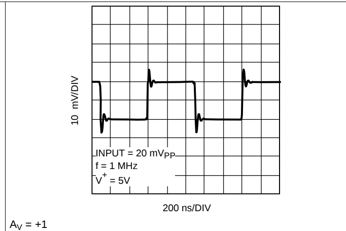
Figure 38. Small Signal Transient Response
