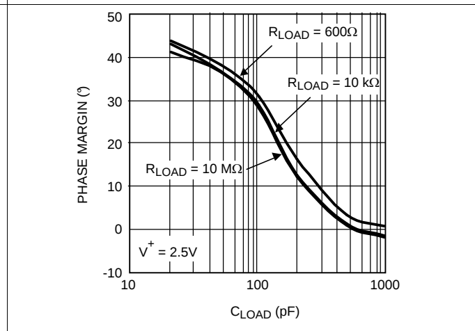
Figure 40. Phase Margin vs Capacitive Load (Stability)
