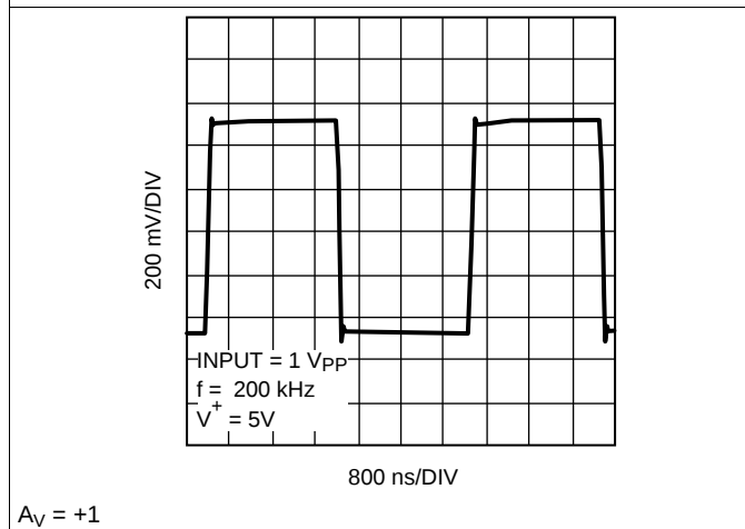
Figure 39. Large Signal Transient Response
