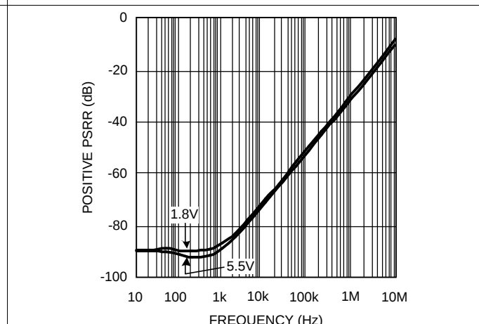
Figure 42. Positive PSRR vs Frequency
