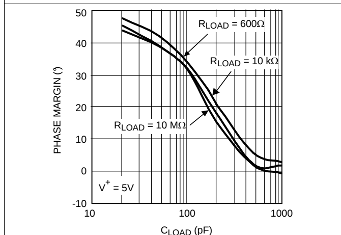
Figure 41. Phase Margin vs Capacitive Load (Stability)
