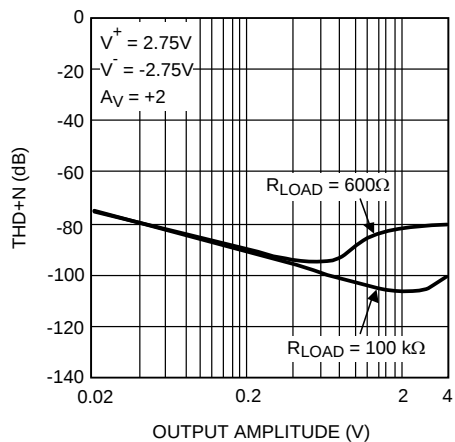
Figure 29. THD+N vs Peak-to-Pek Output Voltage ( V_{OUT} )
