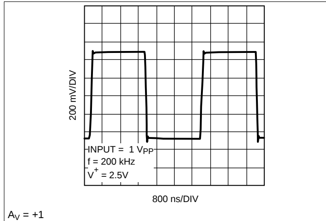
Figure 37. Large Signal Transient Response
