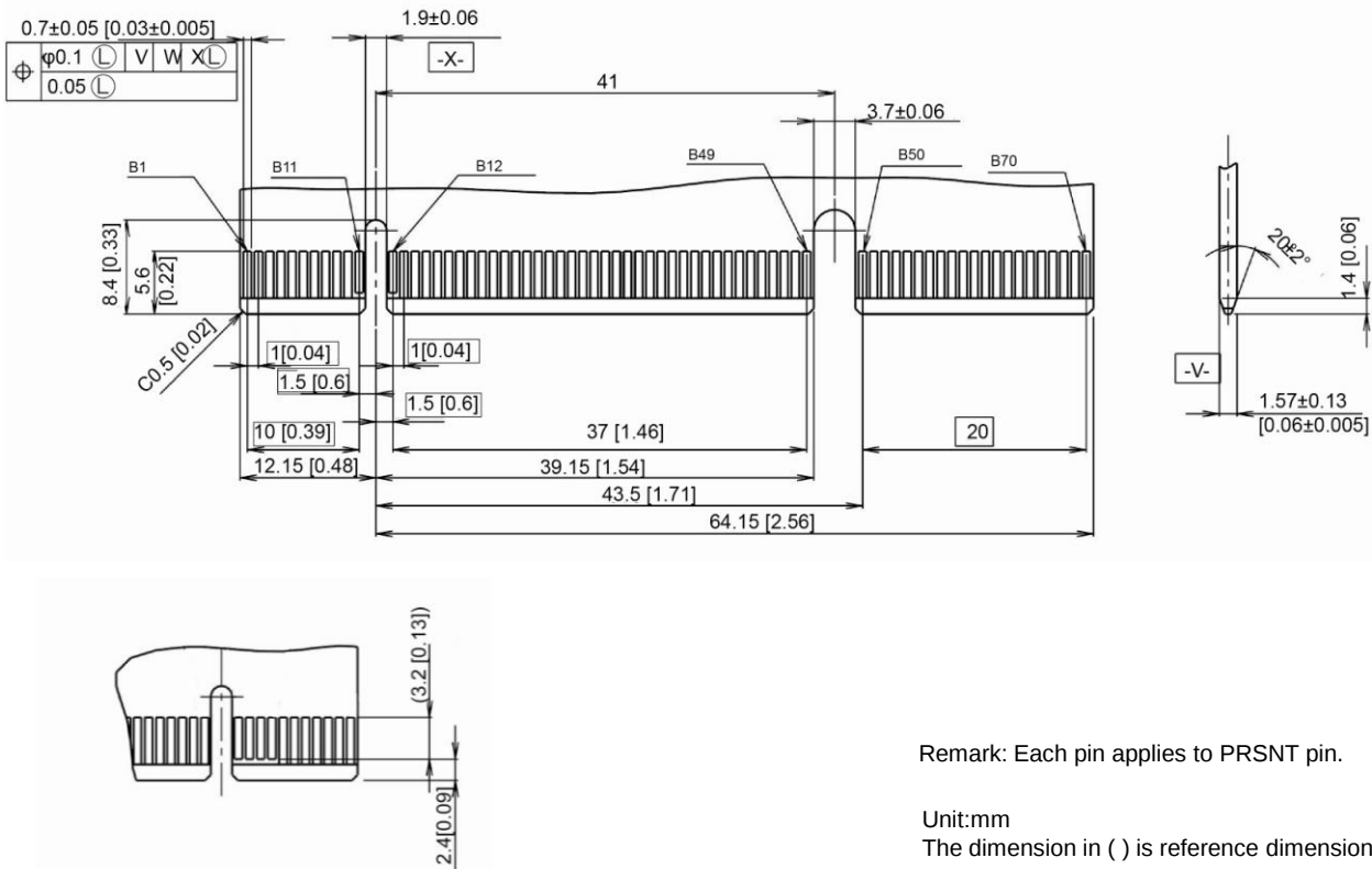
[12 lane 140 contacts module]
