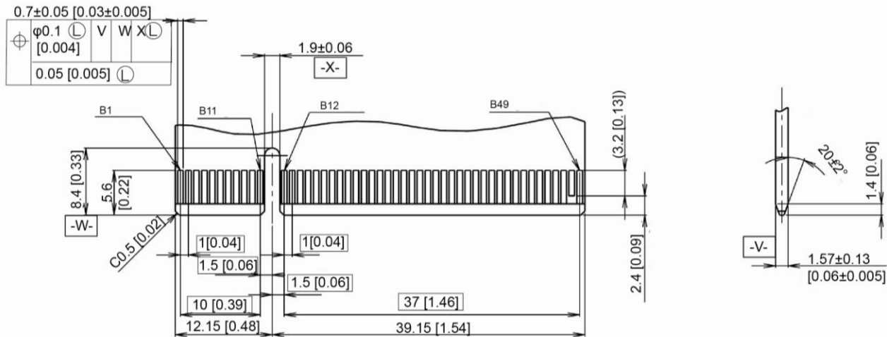
[8 lane 98contacts module]
