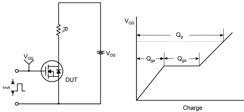
Figure 12. Gate Charge Test Circuit & Waveform
