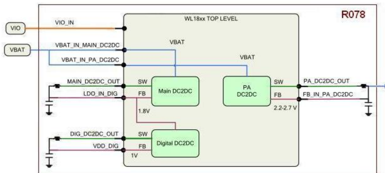
Figure 3-5 Internal DC2DC's
