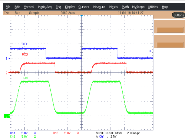
Figure 10-6. LIN Bus Performance
