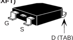
TO-268 (IXFT)
