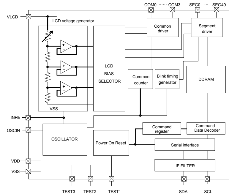
Figure 2. Block Diagram
