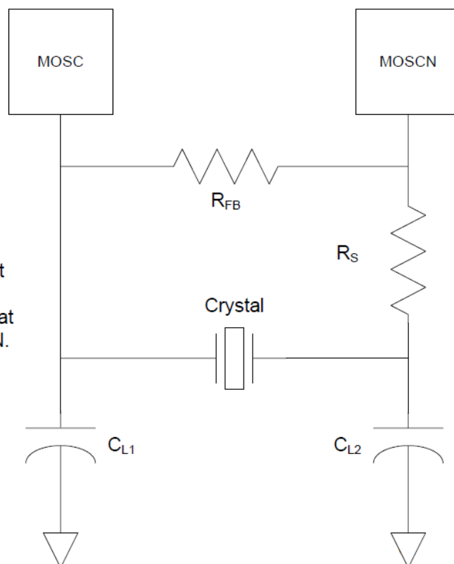
Figure 13. Recommended Crystal Oscillator Configuration
