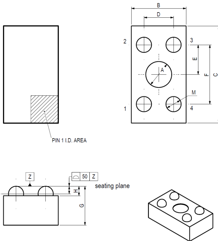
Figure 10 Package outline drawing of the SHTW2.
