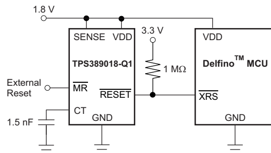
Figure 25. TPS3890-Q1 Monitoring the Supply Voltage for a Delfino Microprocessor
