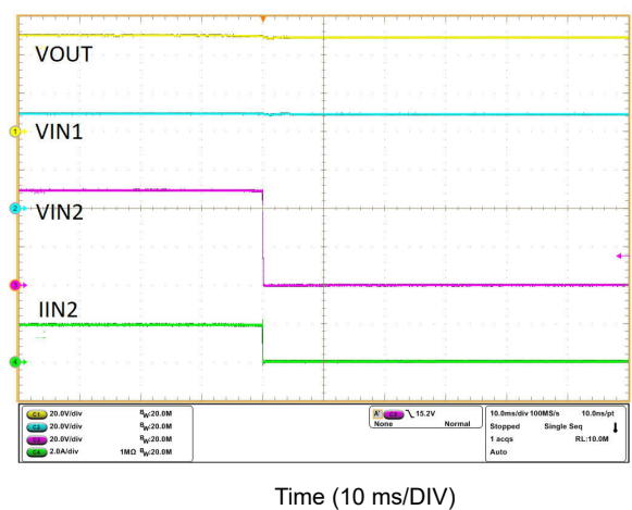
Figure 10-17. OR-ing - V_{IN2} Failure and Switch Over to V_{IN1}
