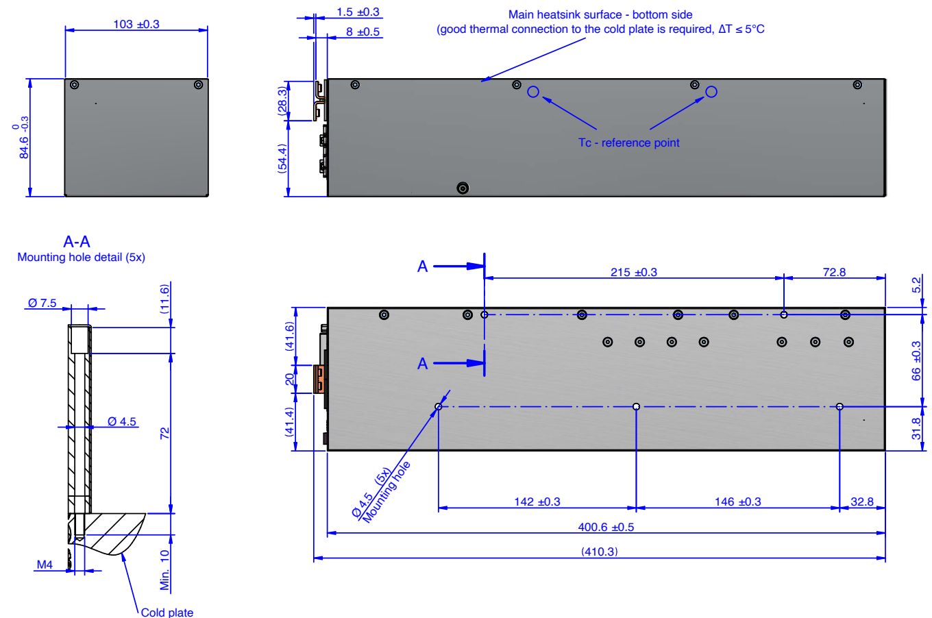
Figure 3. Mechanical Drawing
