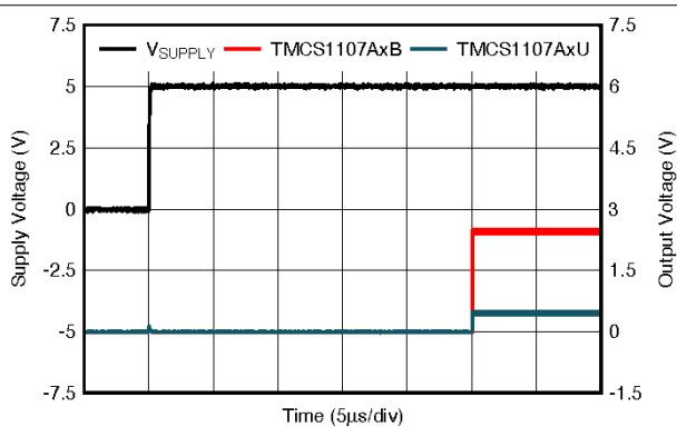
Figure 7-12. Startup Transient Response
