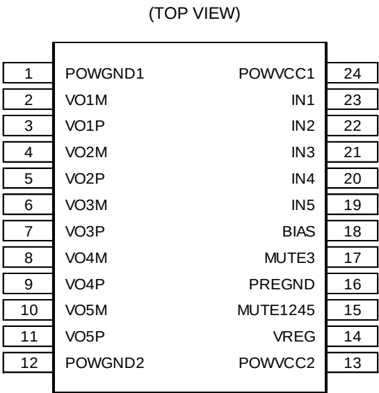
Figure 2. Pin Configuration
