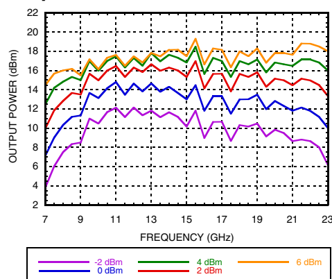
Output Power vs. Drive Level
