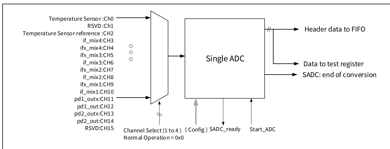
Figure 79 SADC Integration
