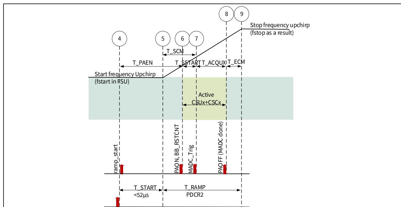
Figure 18 T_RAMP timing conditions
