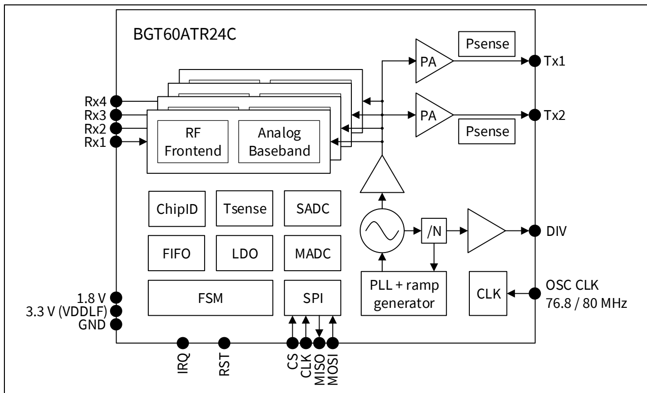
Figure 2 BGT60ATR24C Bare die block diagram
