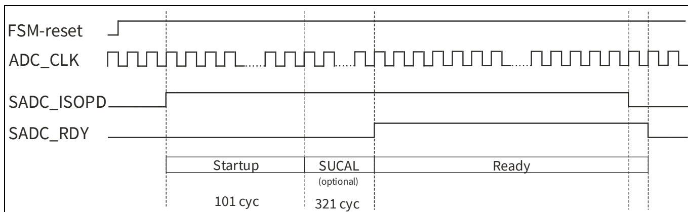
Figure 80 SADC startup timing
