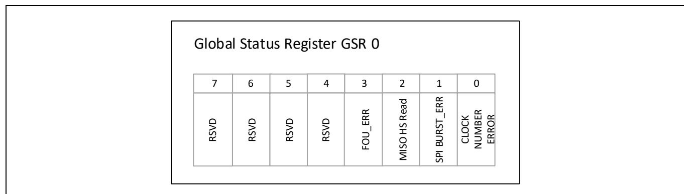
Figure 45 GSR0 Register
