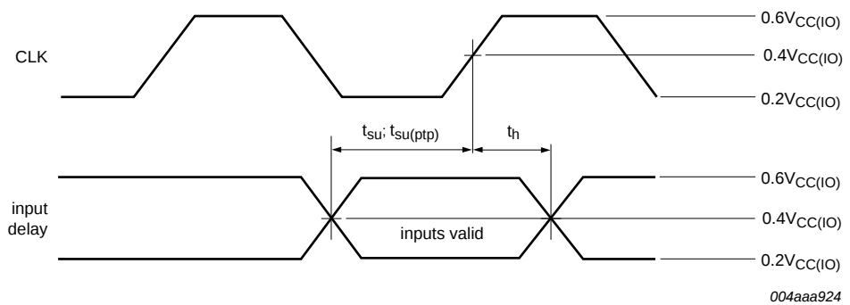
Fig 11. PCI input timing
