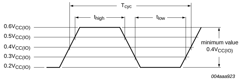
Fig 10. PCI clock
