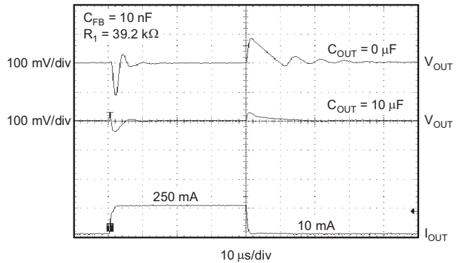
Figure 34. TPS73233 Load Transient Response
