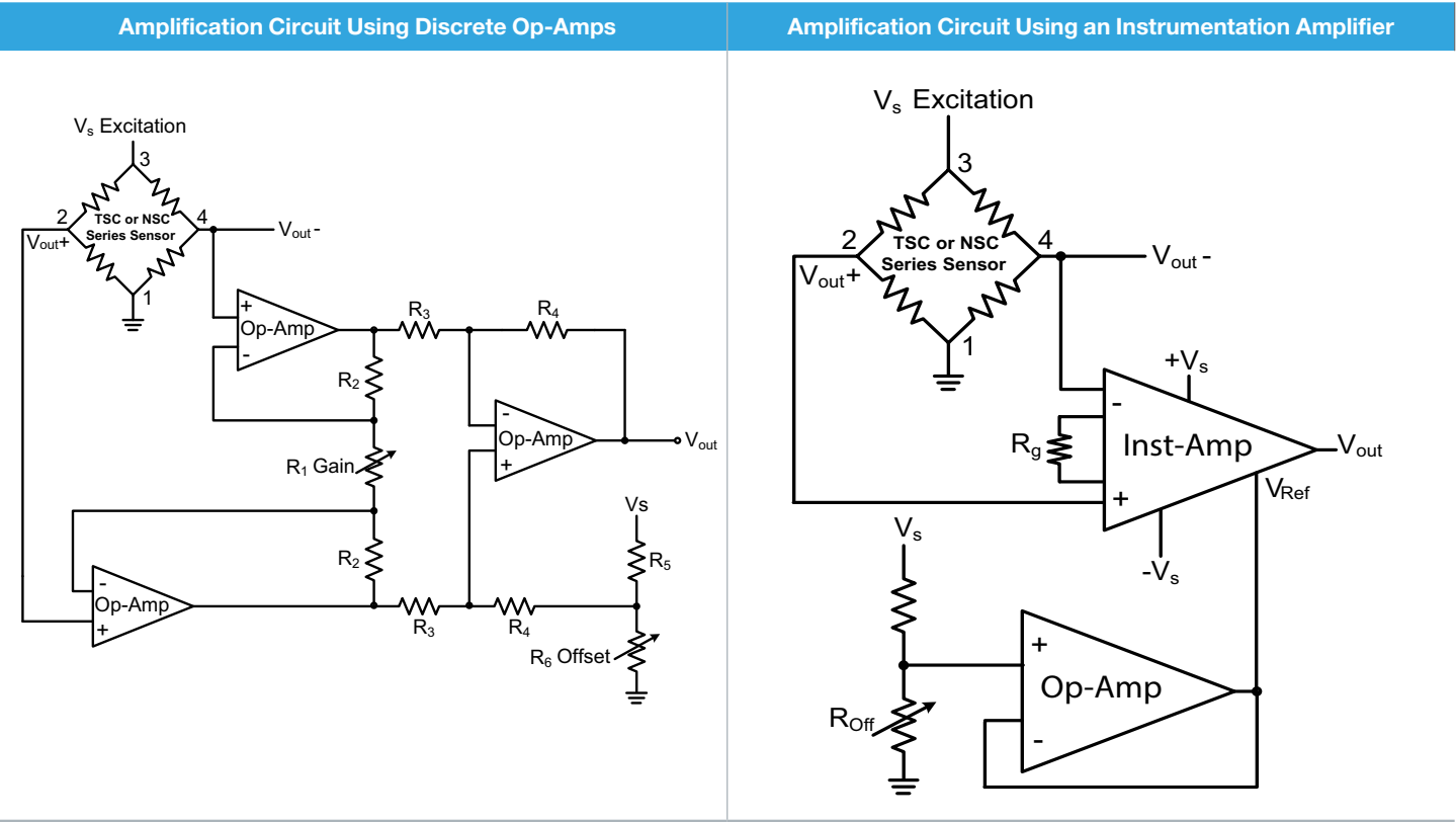
Figure 9. Circuit Examples
