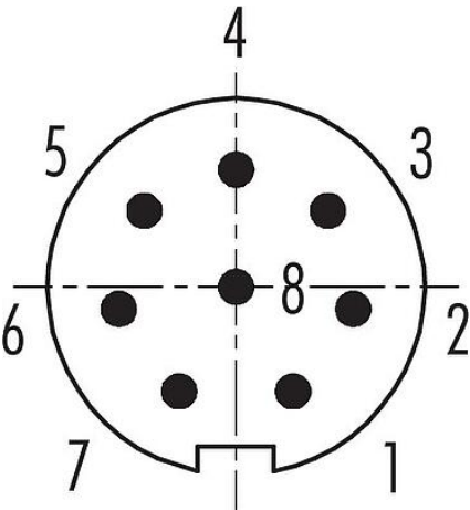
Contact arrangement (Plug-in side)
