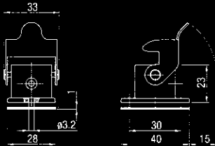
Montageausschnitt/Panel cut-out 22 x22
