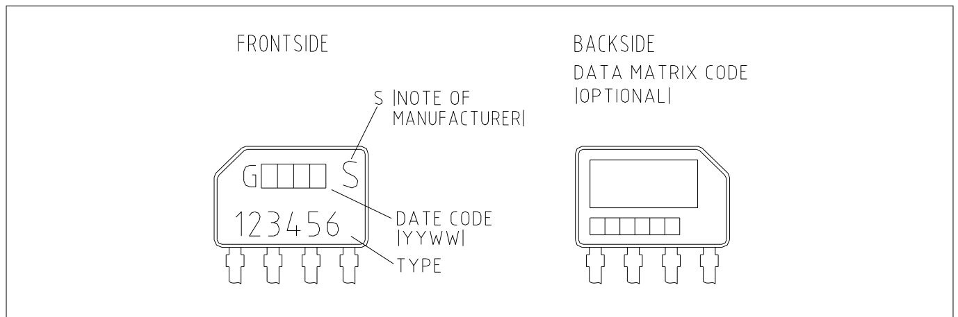
Figure 7 Marking of PG-SSO-4-1 Package
