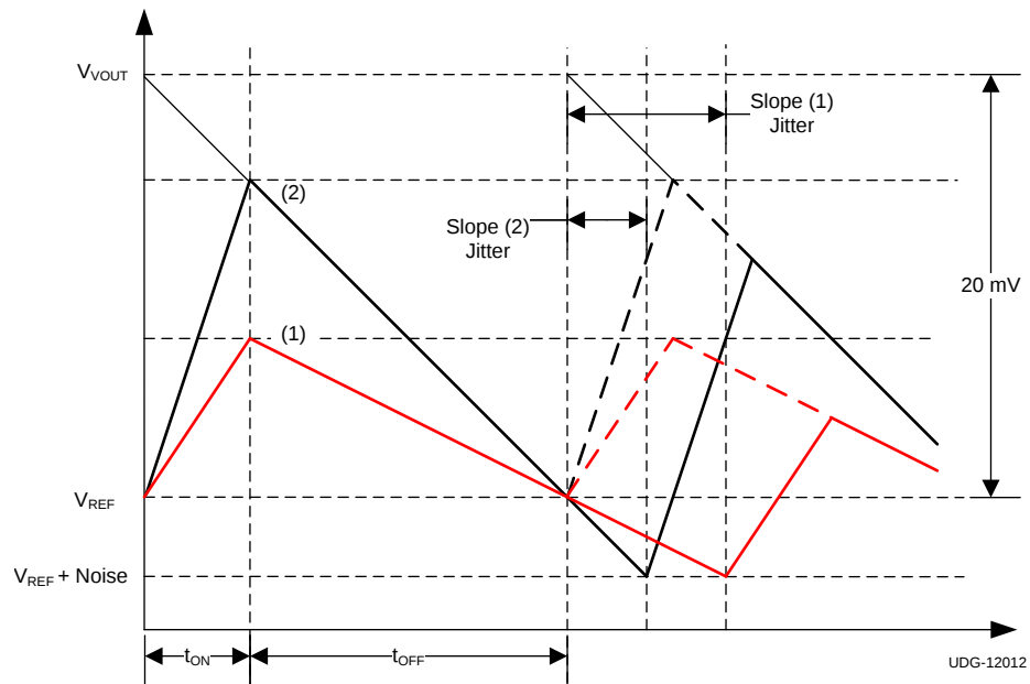
Figure 19. Ripple Voltage Slope and Jitter Performance
