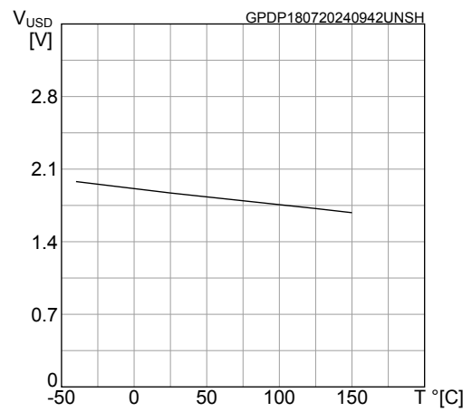
Figure 16. Undervoltage shutdown
