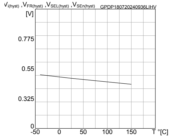
Figure 14. Logic input hysteresis voltage
