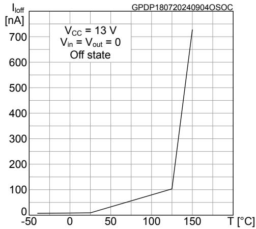
Figure 7. OFF-state output current
