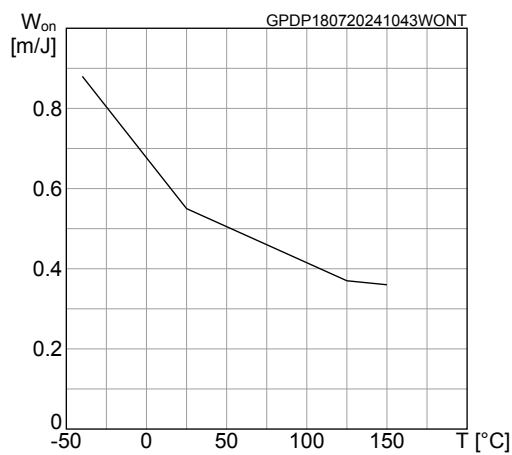
Figure 21. W_{on} vs T_C
