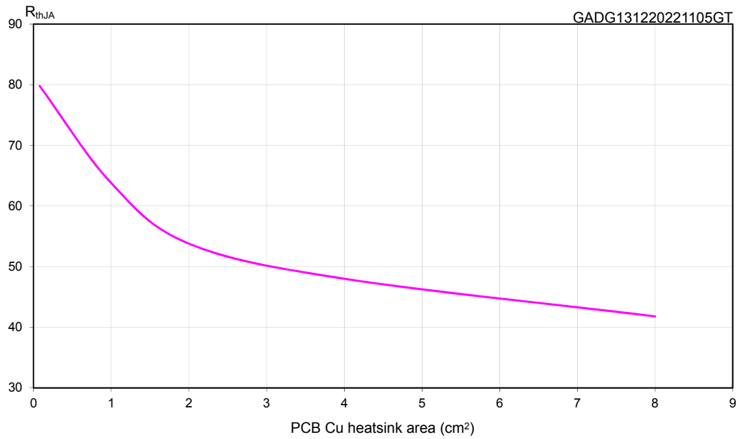
Figure 43. R_{thJA} vs PCB copper area in open box free air condition (one channel on)
