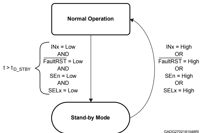
Figure 31. Standby state diagram
