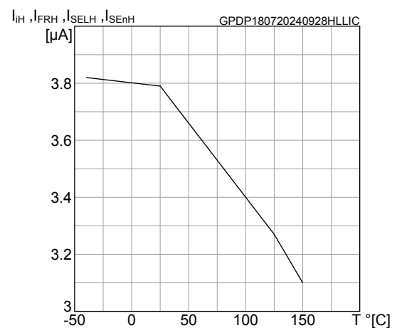
Figure 12. High level logic input current
