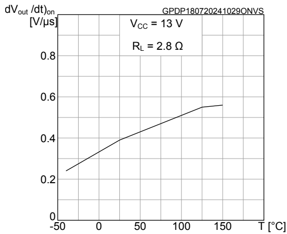
Figure 19. Turn-on voltage slope
