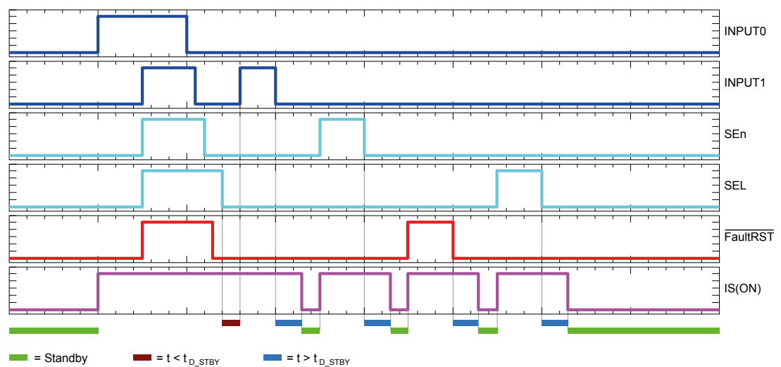
Figure 30. Standby mode activation
