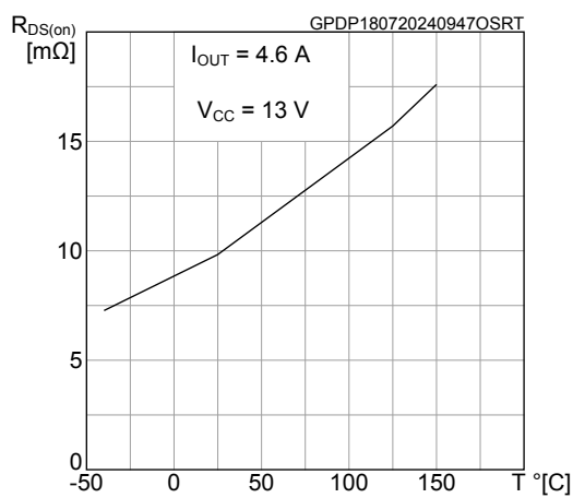
Figure 17. On-state resistance vs. T_C
