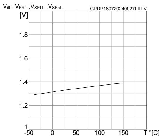
Figure 11. Logic input low level voltage
