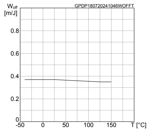
Figure 22. W_{off} vs T_C
