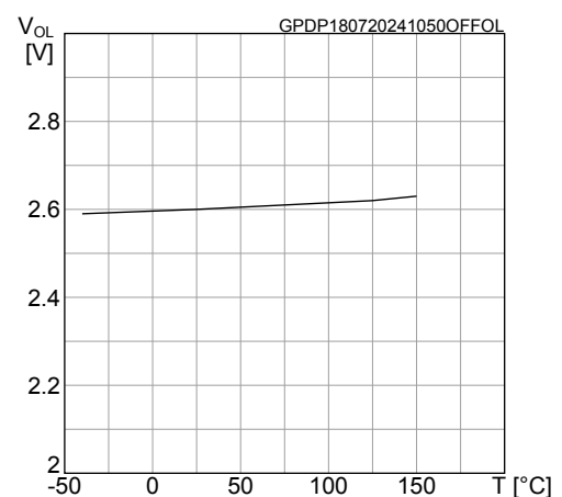
Figure 24. OFF-state open-load voltage detection threshold
