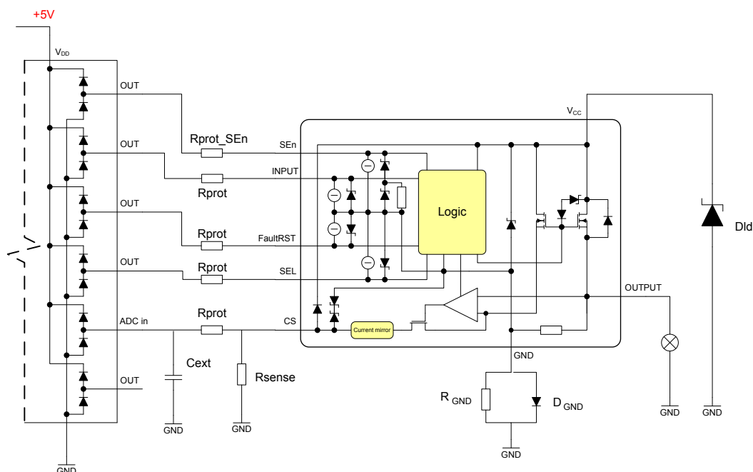
Figure 32. Application diagram
