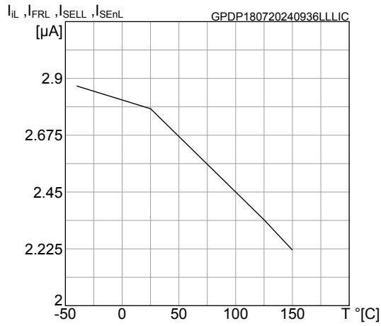
Figure 13. Low level logic input current
