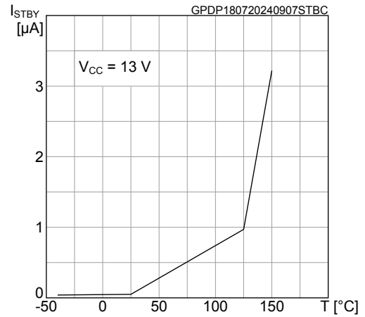
Figure 8. Standby current
