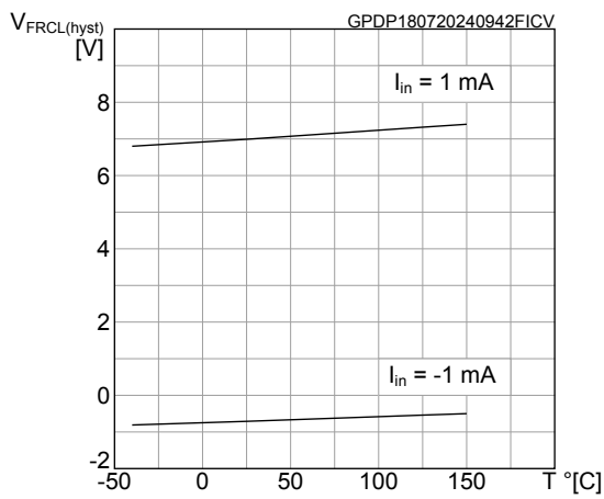
Figure 15. FaultRST input clamp voltage
