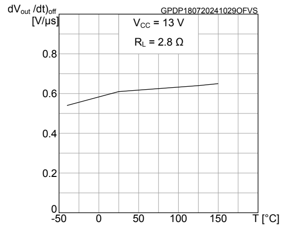
Figure 20. Turn-off voltage slope
