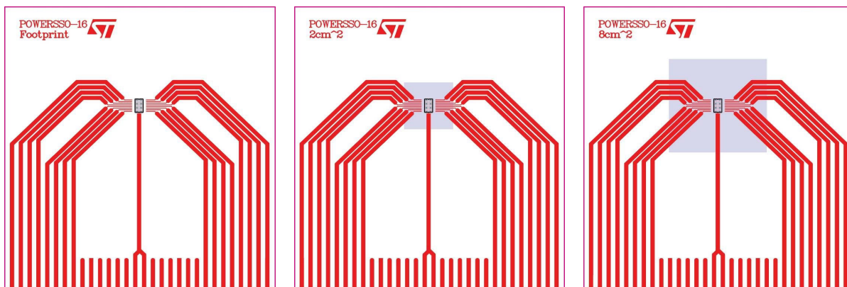
Figure 42. PowerSSO-16 on four-layer PCB (2s2p to JEDEC JESD 51-7)
