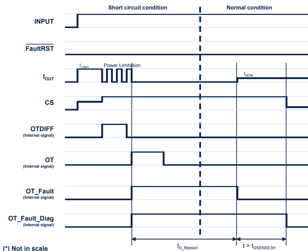
Figure 28. Auto-restart mode - Intermittent short circuit
