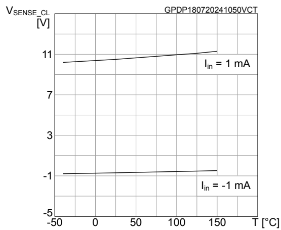
Figure 25. V_{\text{Sense clamp}} vs T_C
