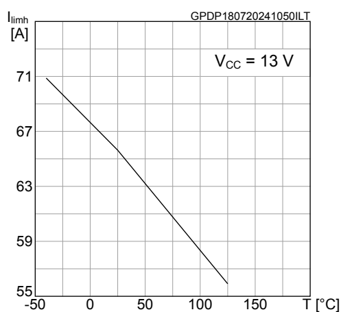
Figure 23. I_{limH} vs T_C
