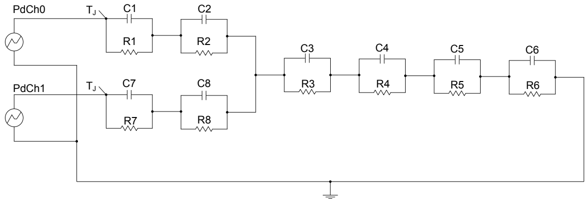
Figure 45. Thermal fitting model of a double-channel HSD in PowerSSO-16
