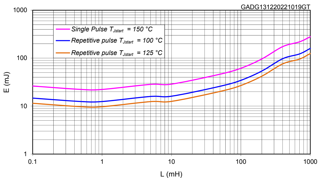
Figure 40. Maximum turn off energy versus inductance
