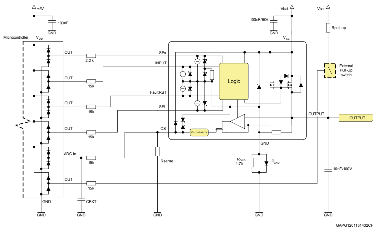
Figure 37. Analog HSD – open-load detection in off-state
