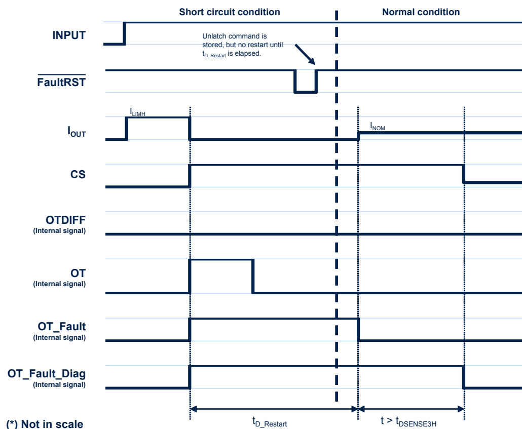
Figure 27. Latch-off mode - Intermittent short circuit
