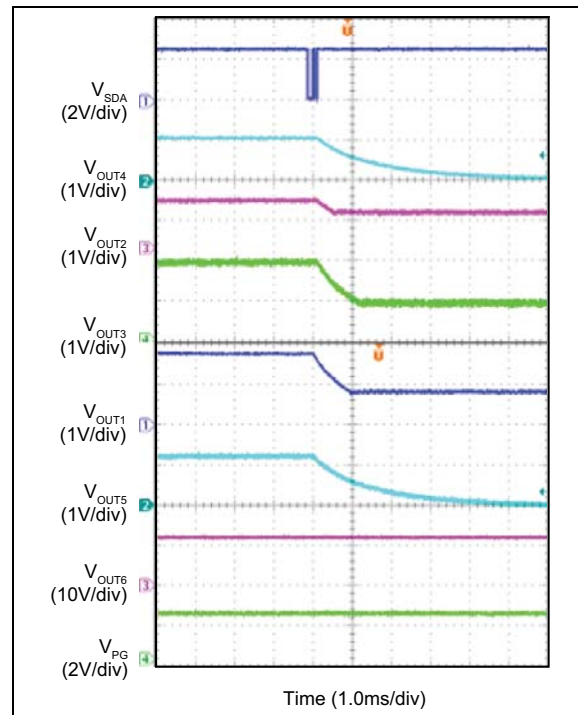
FIGURE 4-12: I 2 C Stand-by Mode.
