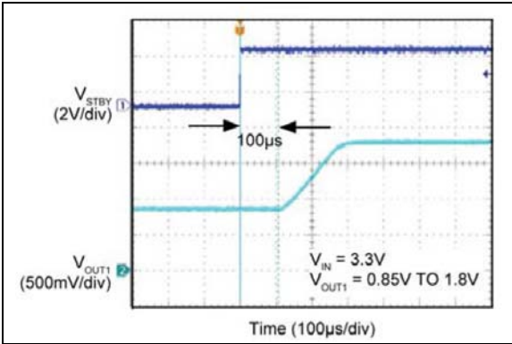
FIGURE 2-22: STBY Delay.
