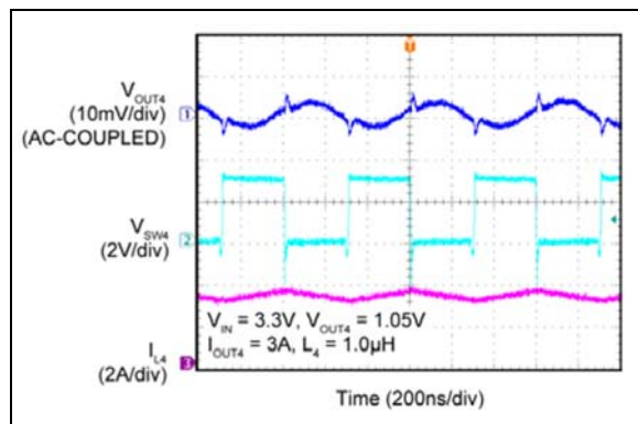
FIGURE 2-41: Buck 4 PWM Switching Waveforms.
