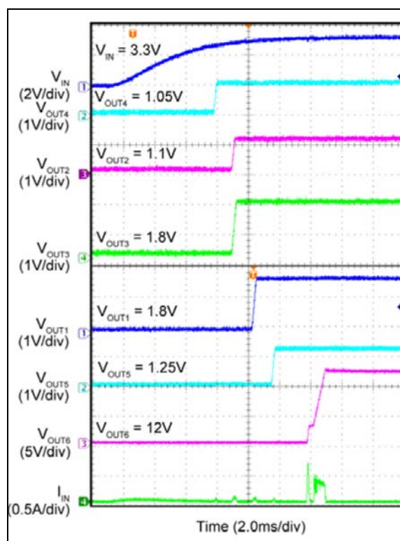
FIGURE 2-45: Input Supply Inrush Current – No Load.
