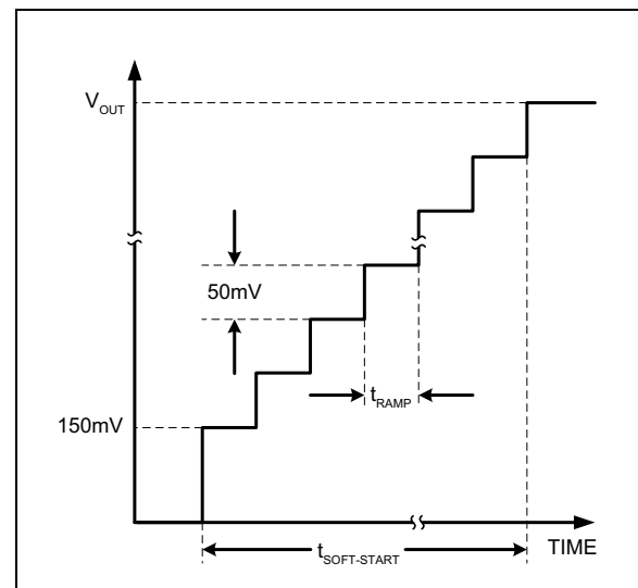
FIGURE 4-1: Buck Soft-Start.
