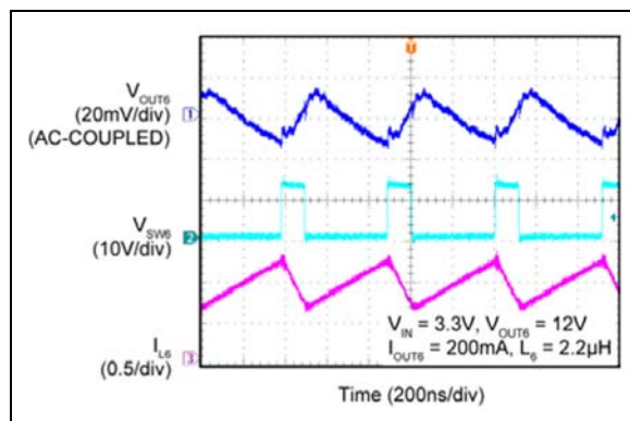
FIGURE 2-43: Boost 6 PWM Switching Waveforms.
