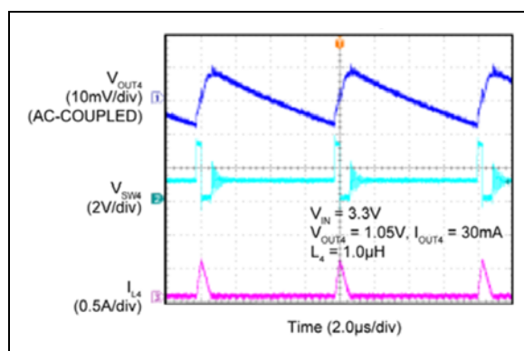
FIGURE 2-42: Buck 4 PFM Switching Waveforms.
