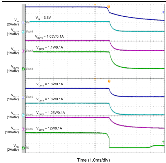
FIGURE 4-11: Hot Unplug – V_{IN} Falling.
