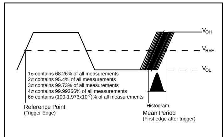
Period Jitter
