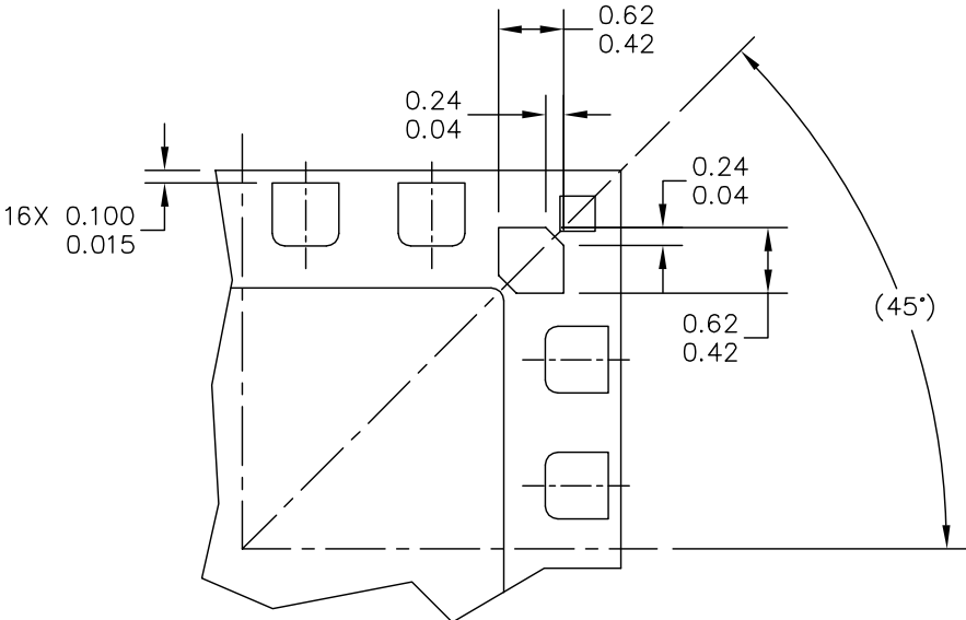
DETAIL M
