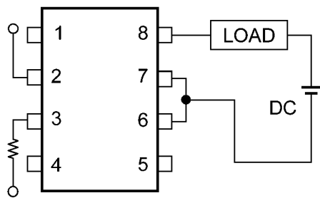
Fig. 14.2.2 B Connection
