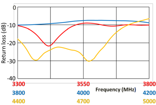
Return Loss
