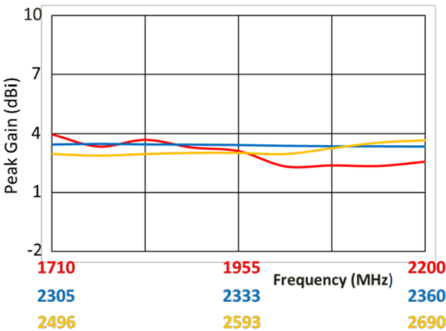
Peak Gain
