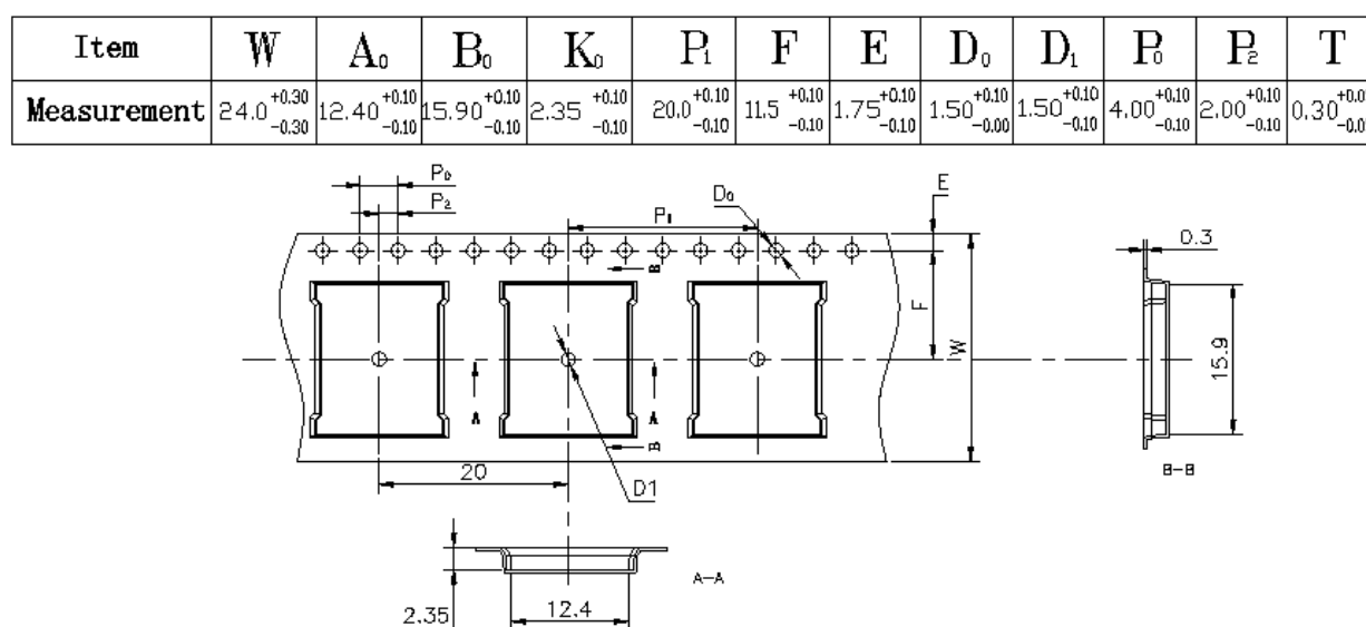
Figure 24. CYBT-343026-01 Tape Dimensions
