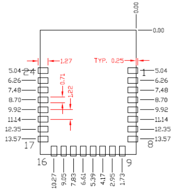
Figure 6. CYBT-343026-01 Host Layout (Relative to Origin)
