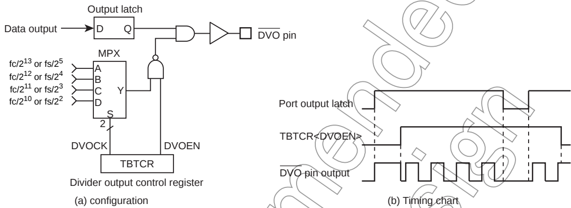
Figure 5-3 Divider Output
