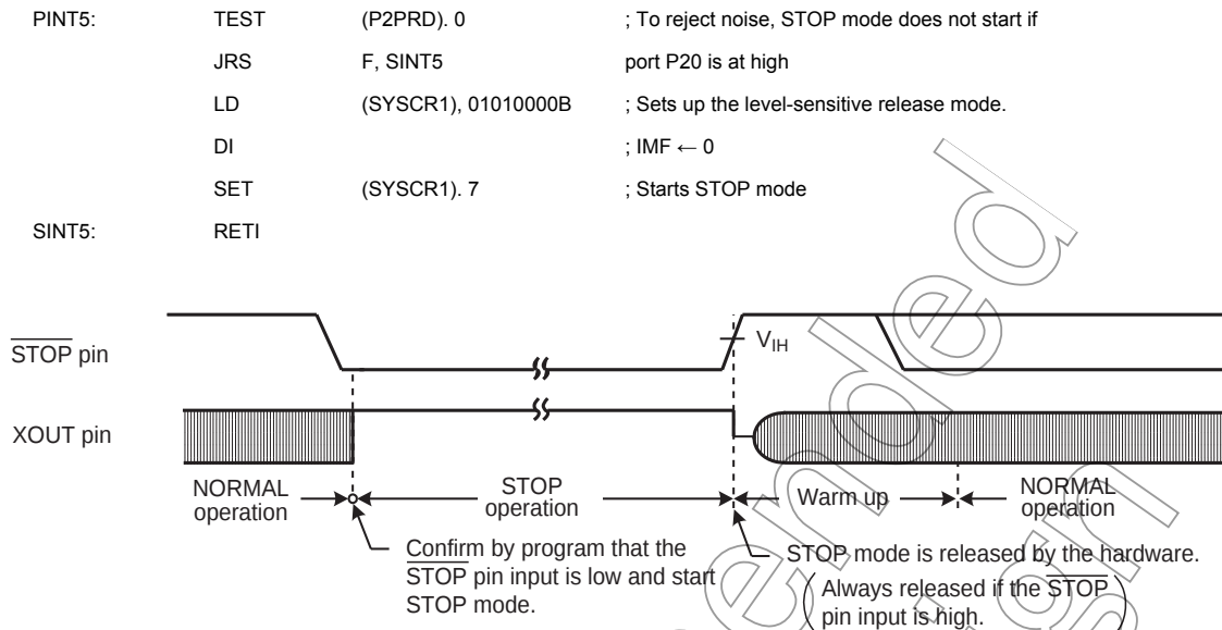
Figure 2-7 Level-sensitive Release Mode
