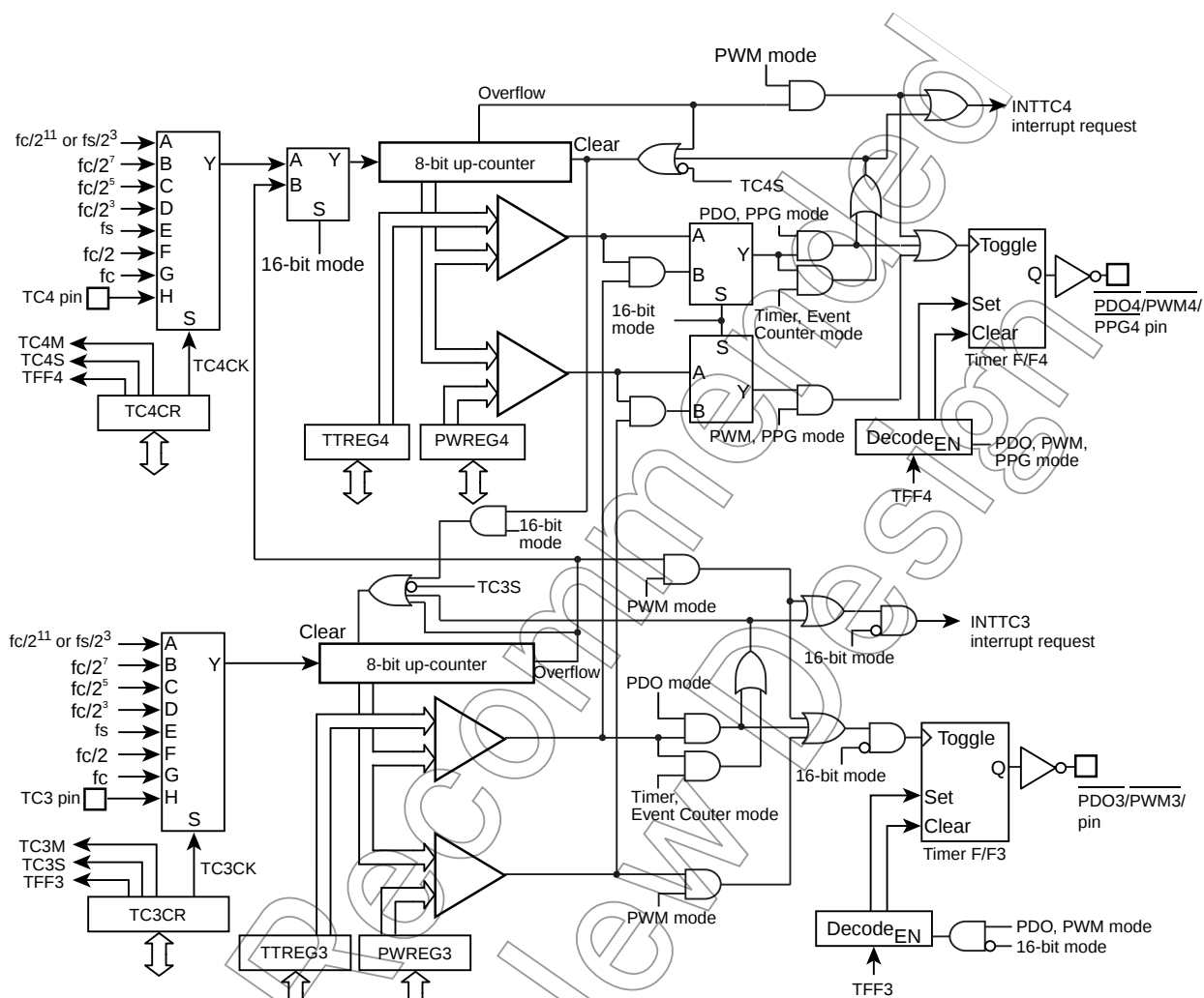
Figure 9-1 8-Bit TimerCounter 3, 4
