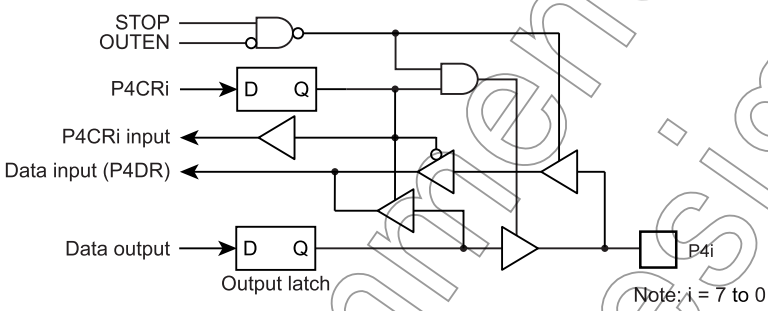
Figure 7-6 Port P4
