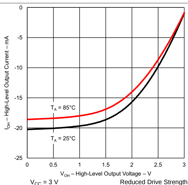
Figure 5-8. High-Level Output Current vs High-Level Output Voltage
