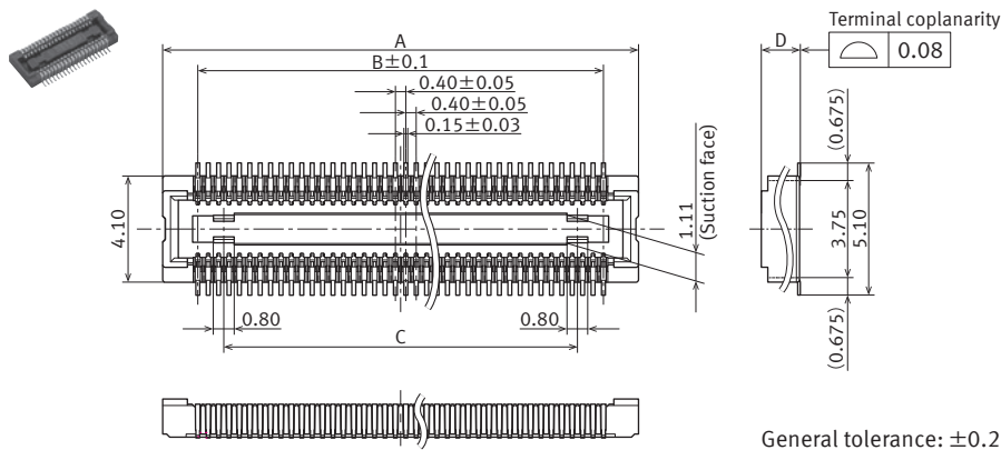
External dimensions
