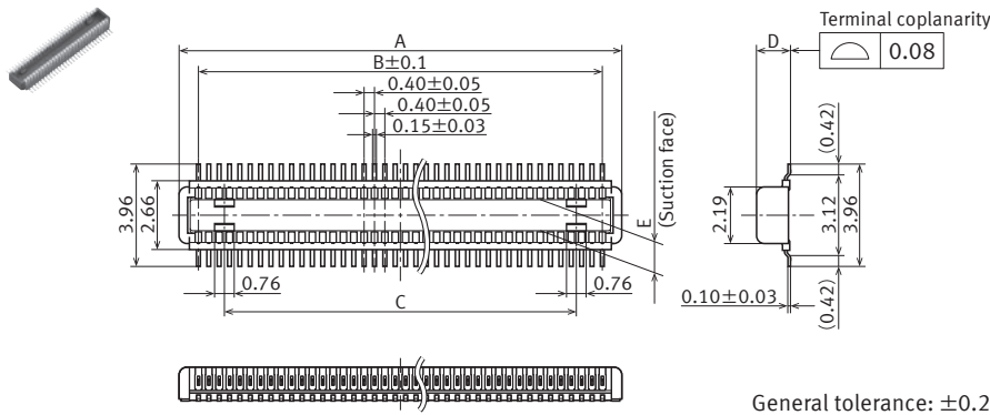
External dimensions
