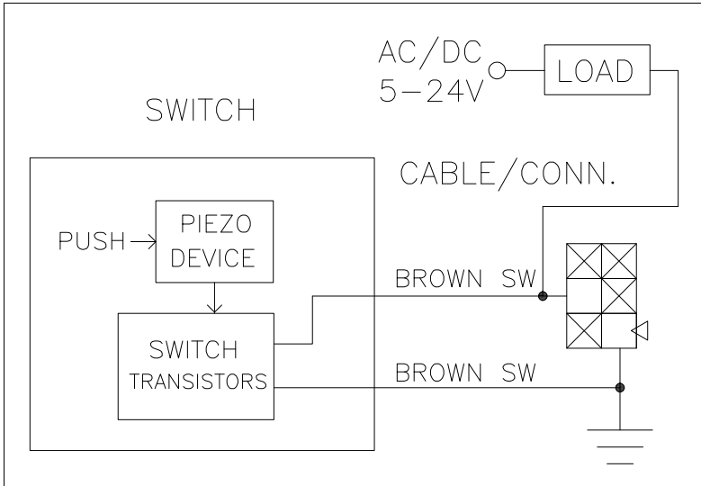
APPLICATION DIAGRAM
