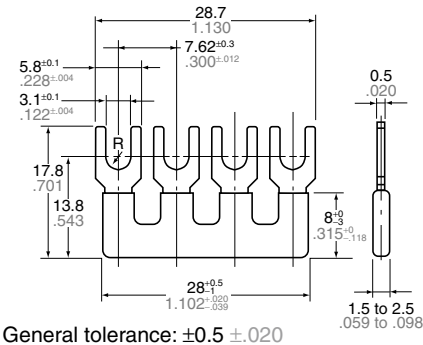
External dimensions (mm inch)
