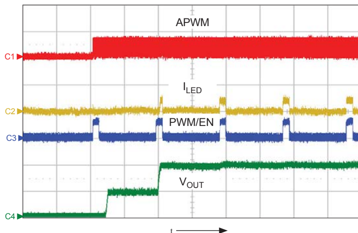
Figure 18. Diagram showing power-up sequencing LED current of 5 mA per channel with a 10% duty cycle PWM signal and a 95% duty cycle APWM signal; shows APWM (ch1, 5 V/div.), I_{LED} (ch2, 50 mA/div.), PWM/EN (ch3, 5 V/div.), and V_{OUT} (ch4, 10 V/div.), time = 500 \mu s/div.
