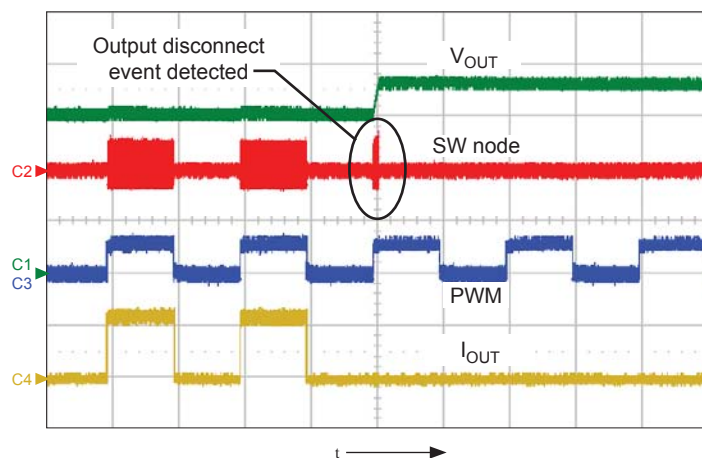
Figure 21. OVP protection in an output disconnect event; shows V_{OUT} (ch1, 10 V/div.), SW node (ch2, 50 V/div.), PWM (ch3, 5 V/div.), and I_{OUT} (ch4, 200 mA/div.), time = 1 ms/div.
