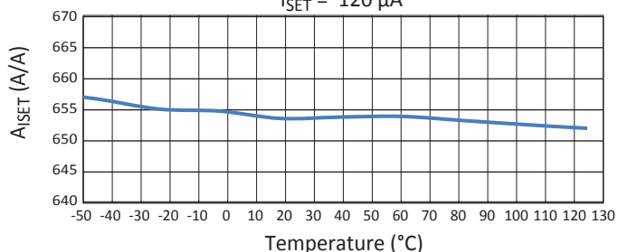
I_{SET} to LED Current Gain versus Ambient Temperature I_{SET} = 120 \mu A
