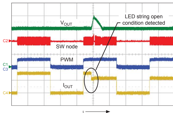
Figure 22. OVP protection in an open LED string event; shows V_{OUT} (ch1, 10 V/div.), SW node (ch2, 50 V/div.), PWM (ch3, 5 V/div.), and I_{OUT} (ch4, 200 mA/div.), time = 500 \mu s/div.
