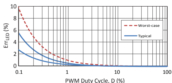
Figure 12. Typical percentage error, due to PWM-to-LED delay, for the average LED current versus PWM duty cycle (at 200 Hz PWM frequency).
