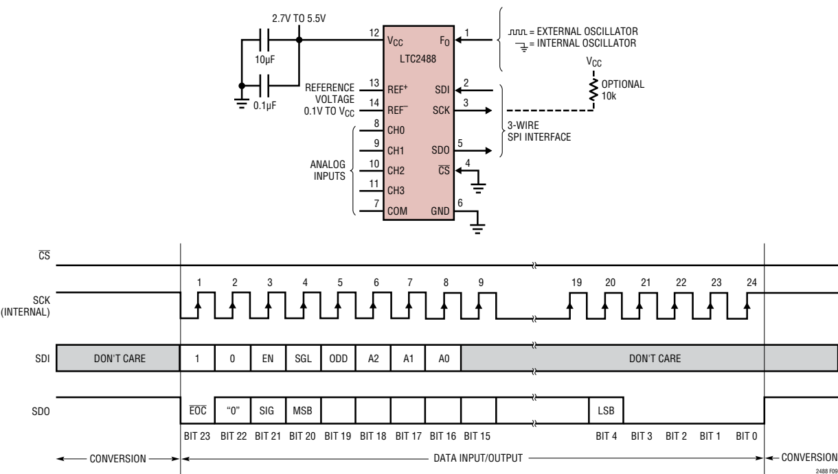
Figure 9. Internal Serial Clock, Continuous Operation
